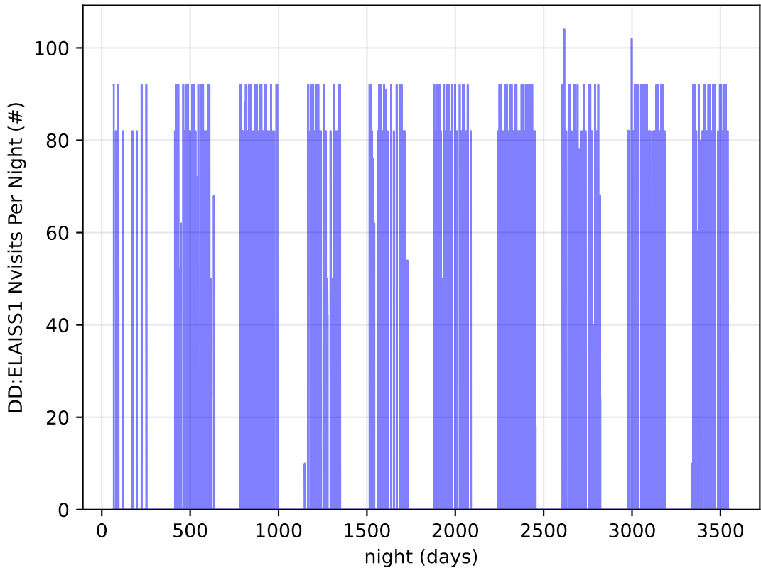
too_elab_r128_d2_gz_v3.4_10yrs all bands: DD:ELAISS1 Nvisits Per Night
