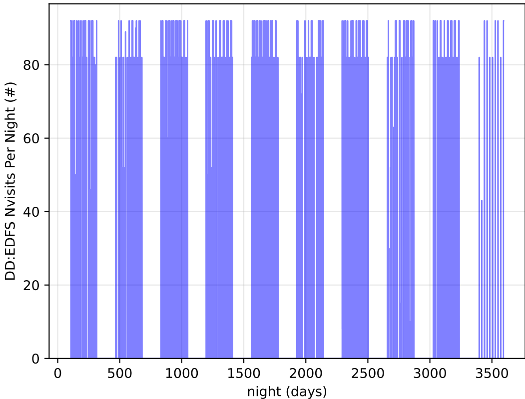
too_elab_r128_d2_gz_v3.4_10yrs all bands: DD:EDFS Nvisits Per Night
