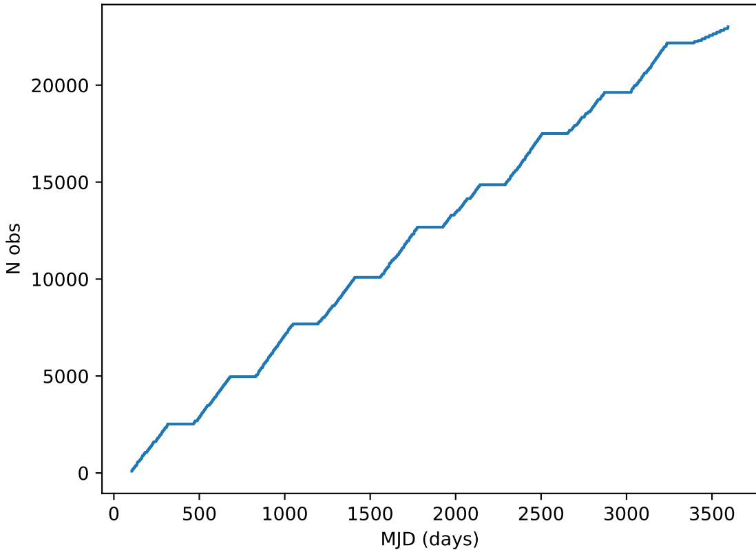
too_elab_r128_d2_gz_v3.4_10yrs all bands: DD:EDFS Cumulative NVisits
