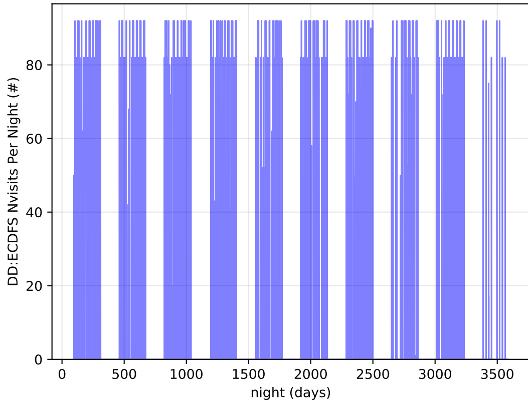
too_elab_r128_d2_gz_v3.4_10yrs all bands: DD:ECDFS Nvisits Per Night
