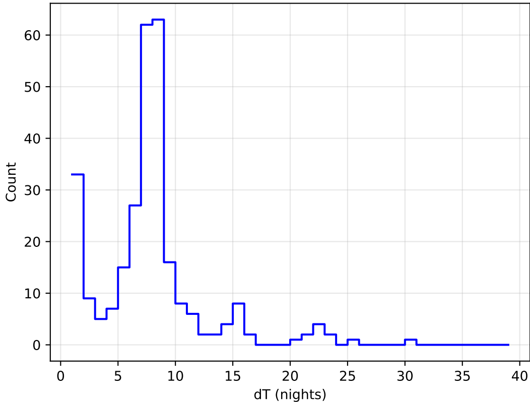
too_elab_r128_d2_gz_v3.4_10yrs all bands: DD:ECDFS Delta Nights Histogram
