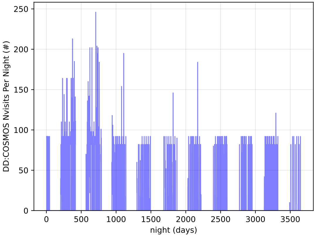
too_elab_r128_d2_gz_v3.4_10yrs all bands: DD: COSMOS Nvisits Per Night
