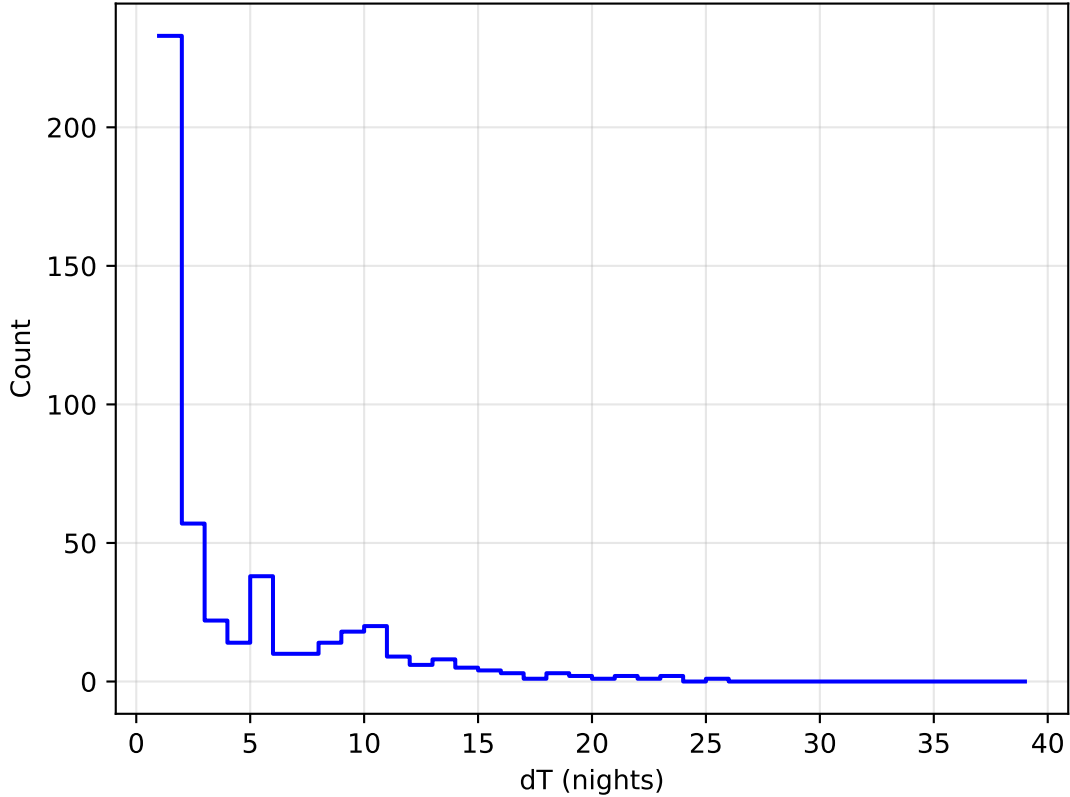
too_elab_r128_d2_gz_v3.4_10yrs all bands: DD: COSMOS Delta Nights Histogram
