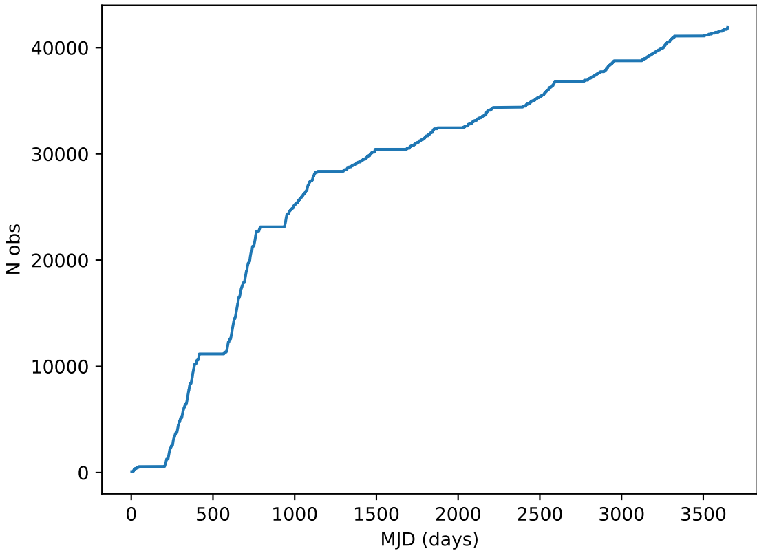
too_elab_r128_d2_gz_v3.4_10yrs all bands: DD: COSMOS Cumulative NVisits
