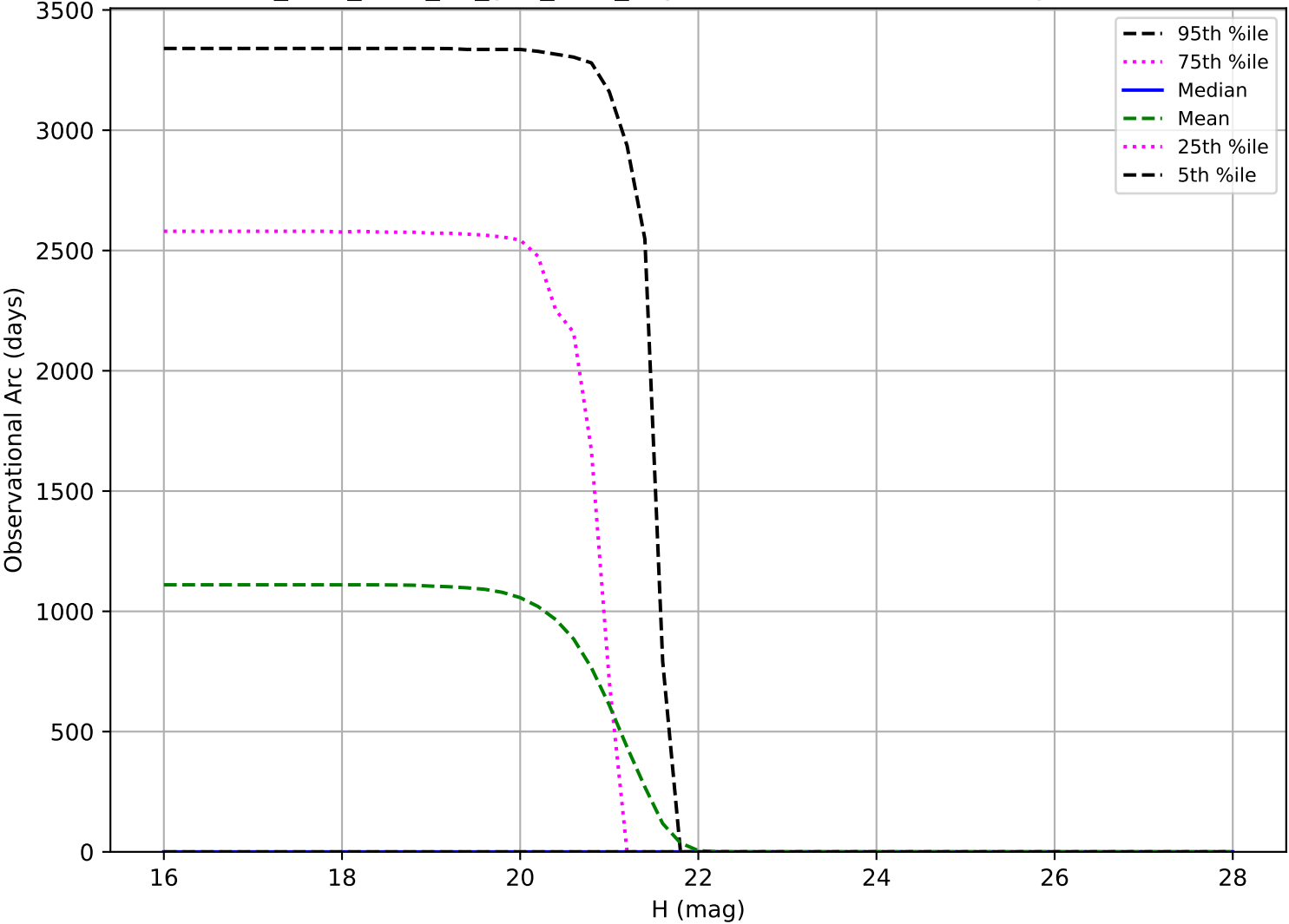
too_elab_r128_d2_griz_v3.4_10yrs: Observational Arc Length Vatra
