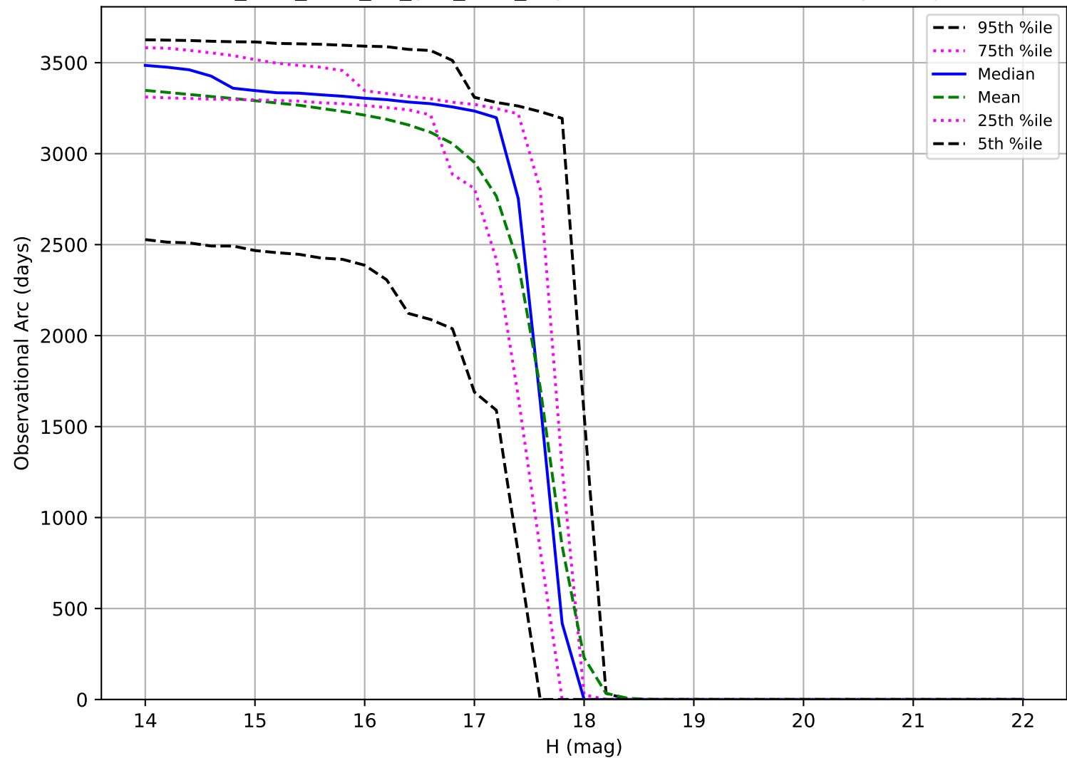
too_elab_r128_d2_griz_v3.4_10yrs: Observational Arc Length Trojan
