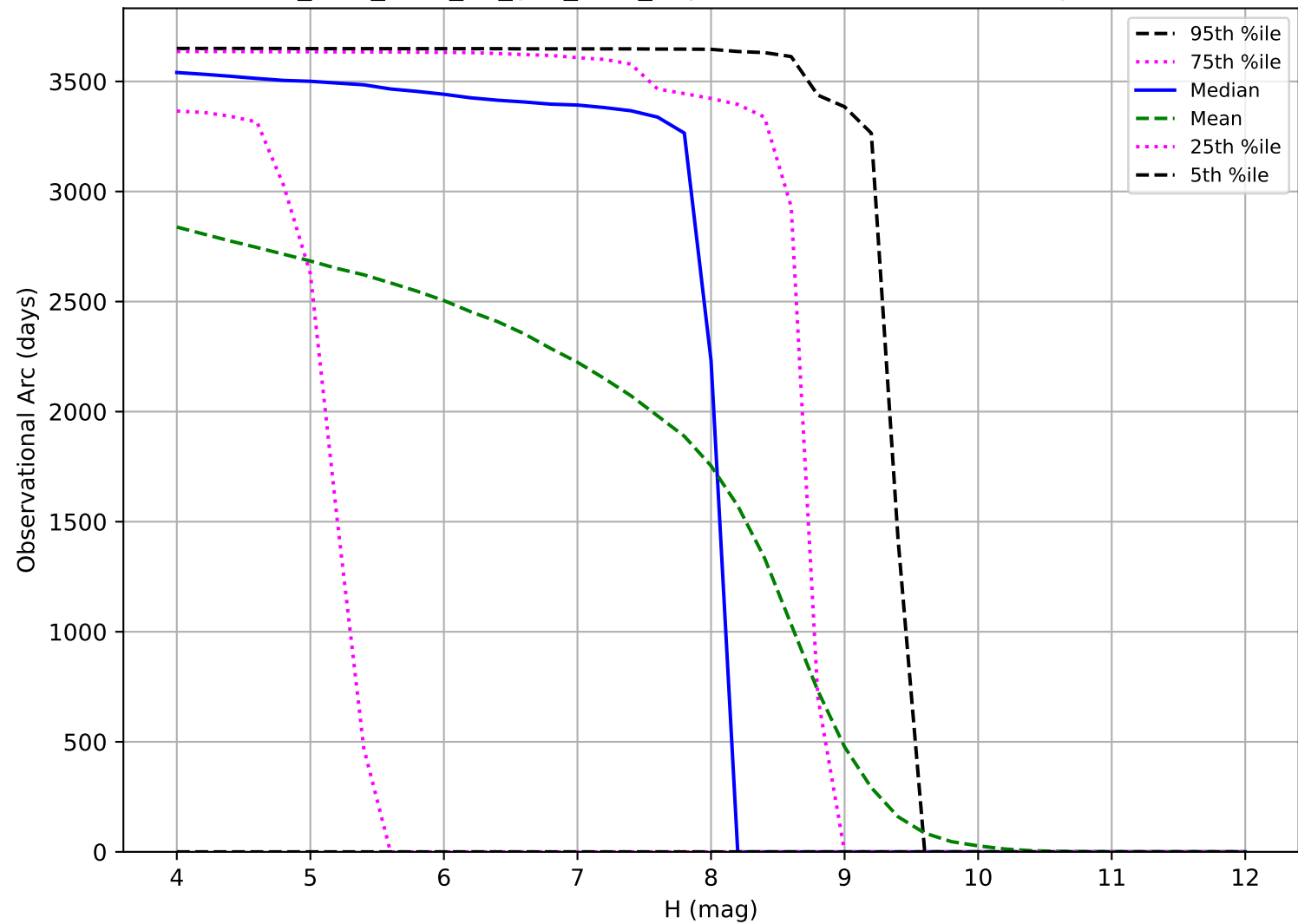
too_elab_r128_d2_griz_v3.4_10yrs: Observational Arc Length TNO
