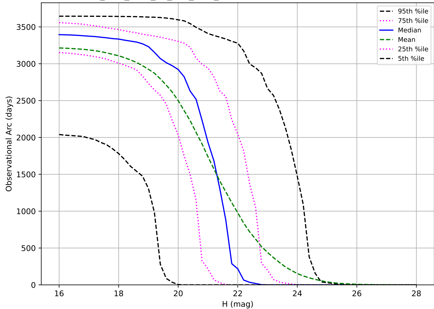
too_elab_r128_d2_griz_v3.4_10yrs: Observational Arc Length PHA
