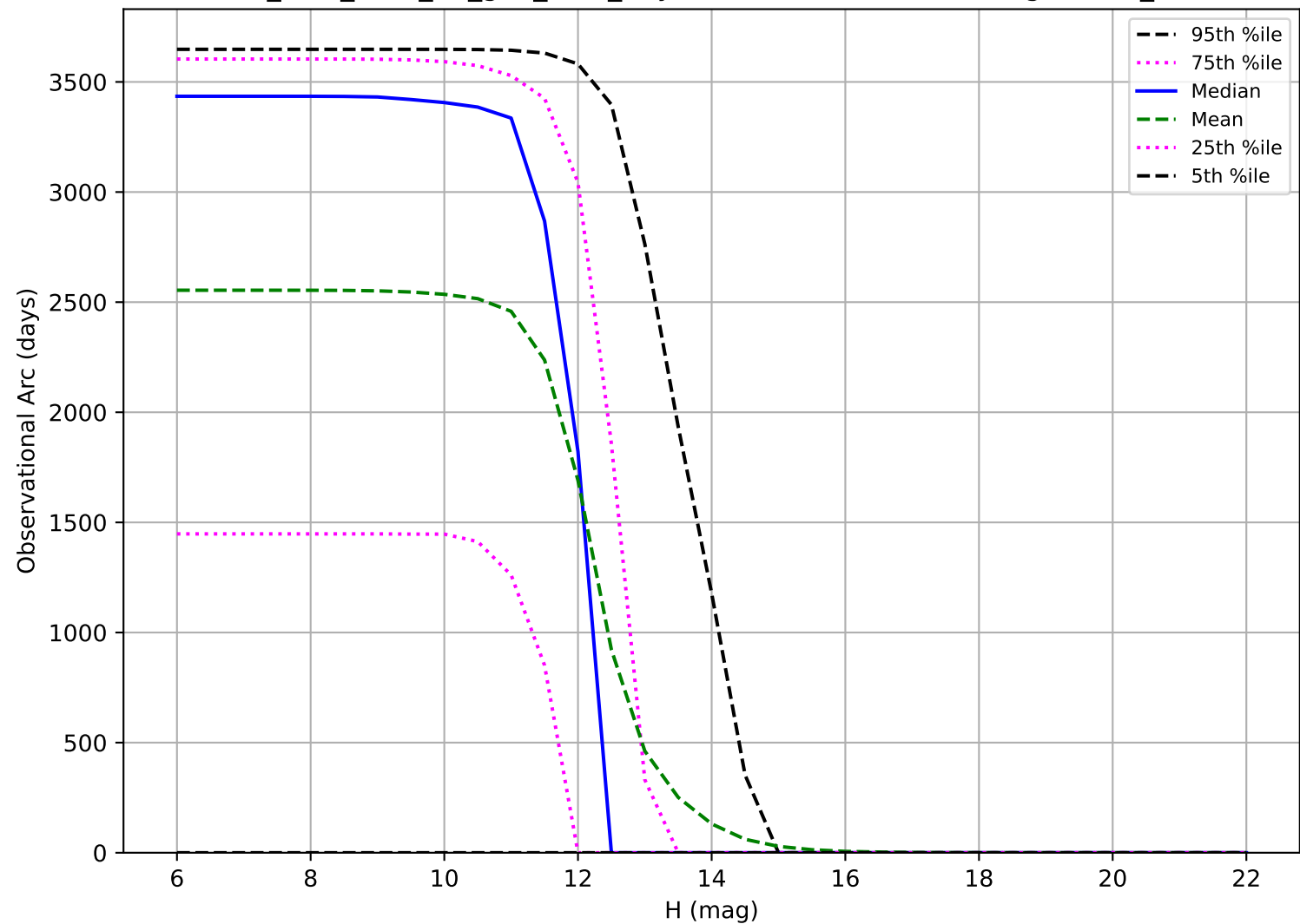
too_elab_r128_d2_griz_v3.4_10yrs: Observational Arc Length OCC_r20
