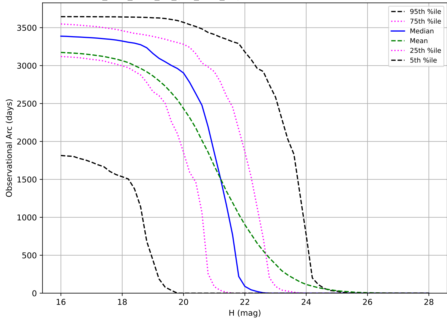
too_elab_r128_d2_griz_v3.4_10yrs: Observational Arc Length NEO
