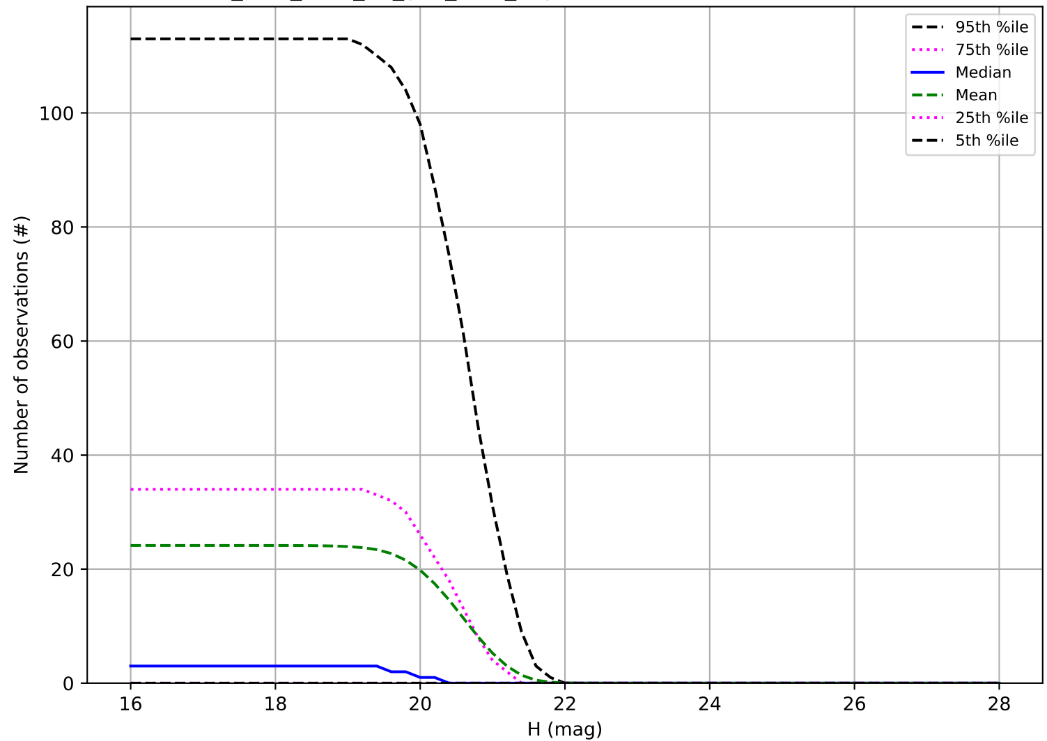
too_elab_r128_d2_griz_v3.4_10yrs: Number of observations Vatira
