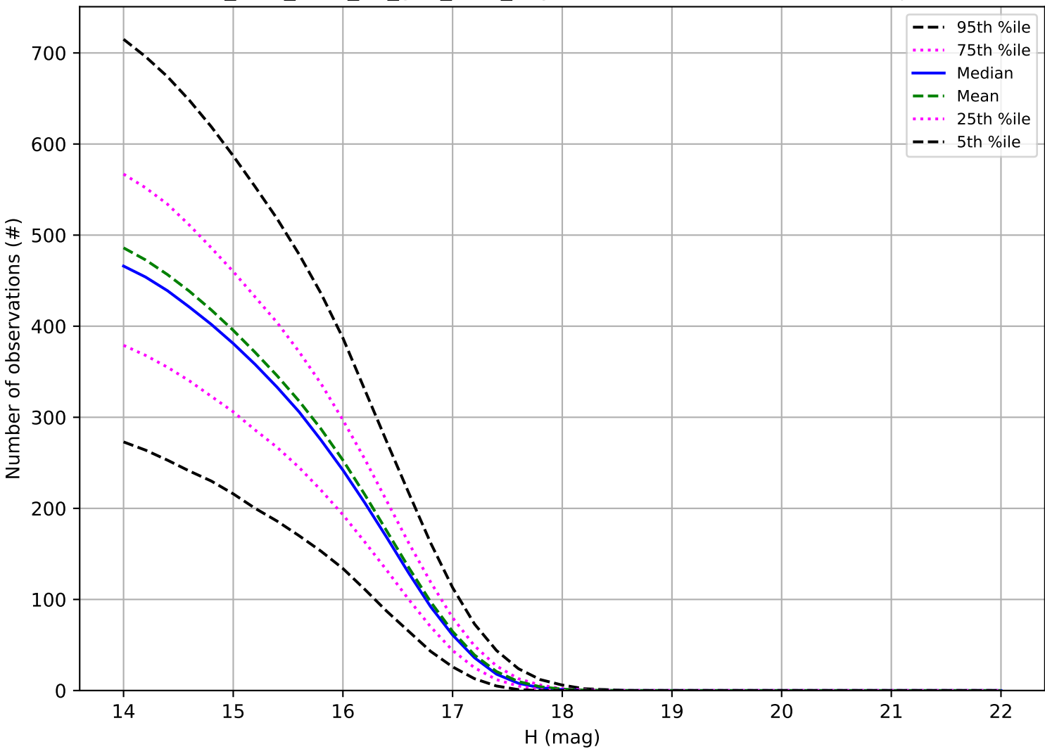
too_elab_r128_d2_griz_v3.4_10yrs: Number of observations Trojan
