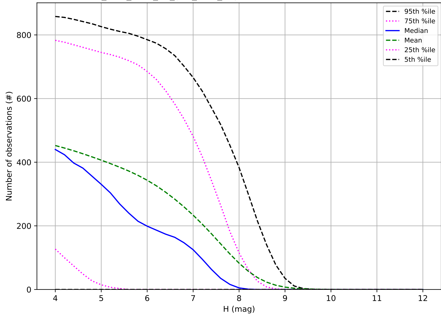
too_elab_r128_d2_griz_v3.4_10yrs: Number of observations TNO
