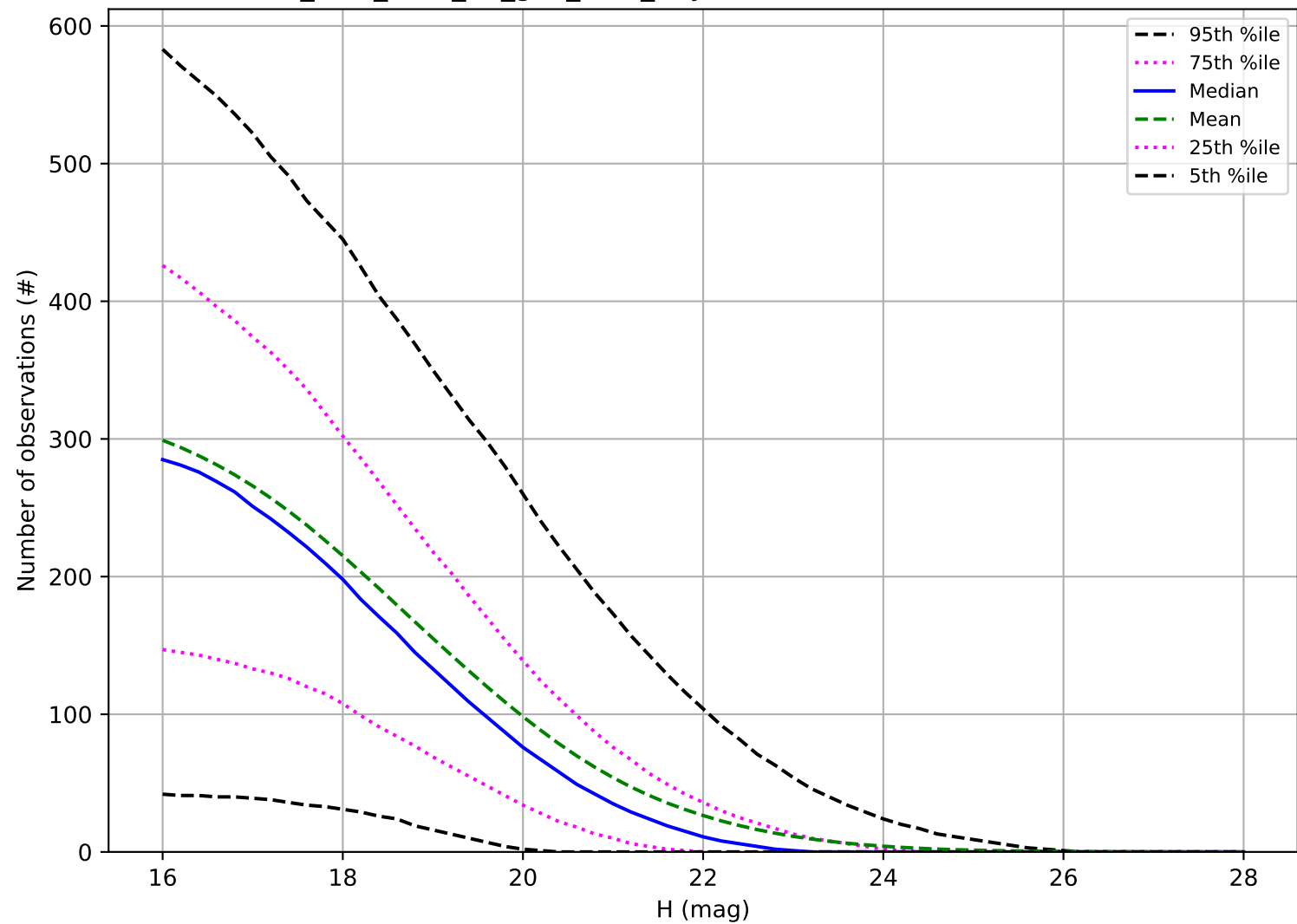
too_elab_r128_d2_griz_v3.4_10yrs: Number of observations PHA
