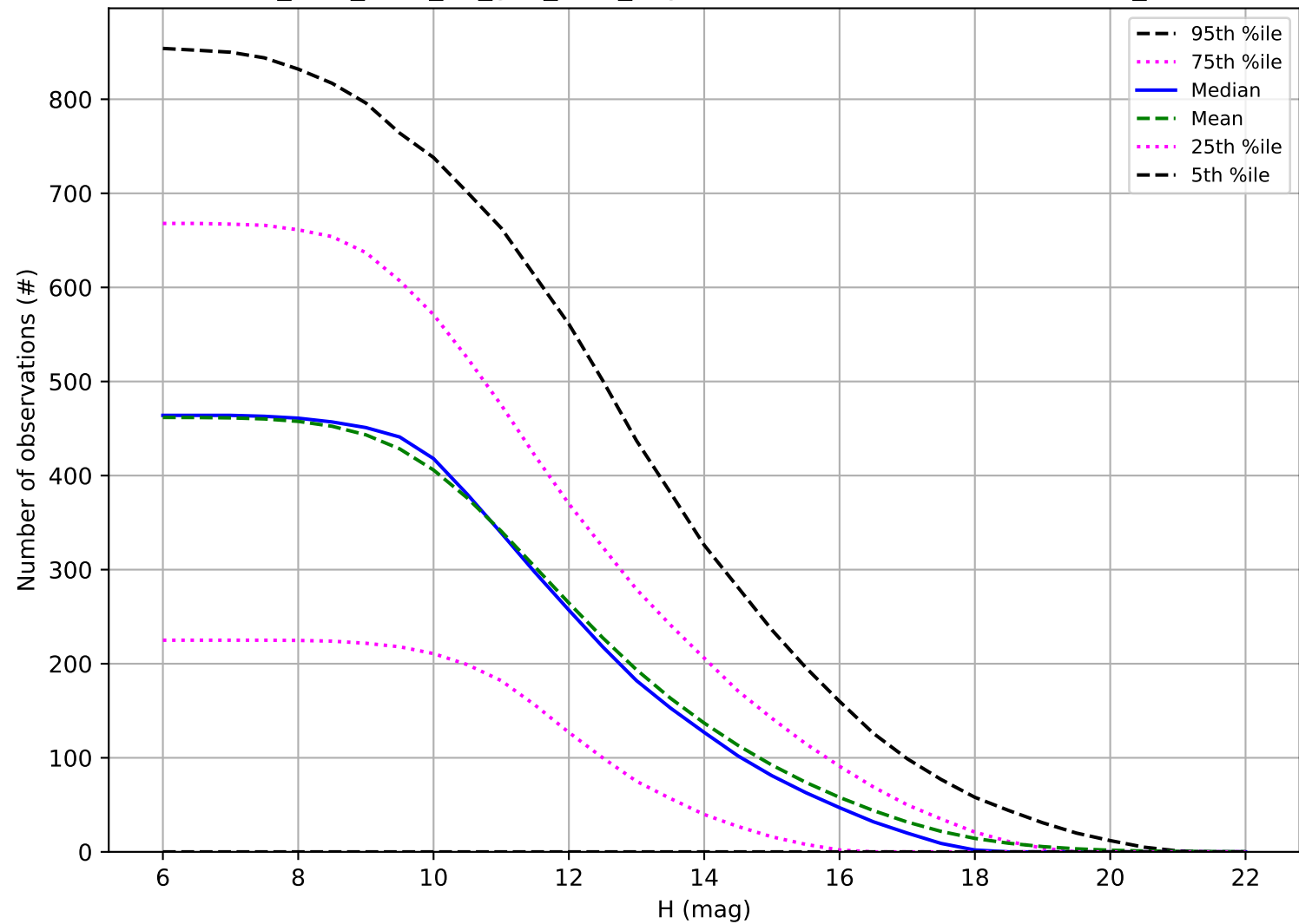
too_elab_r128_d2_griz_v3.4_10yrs: Number of observations OCC_r5
