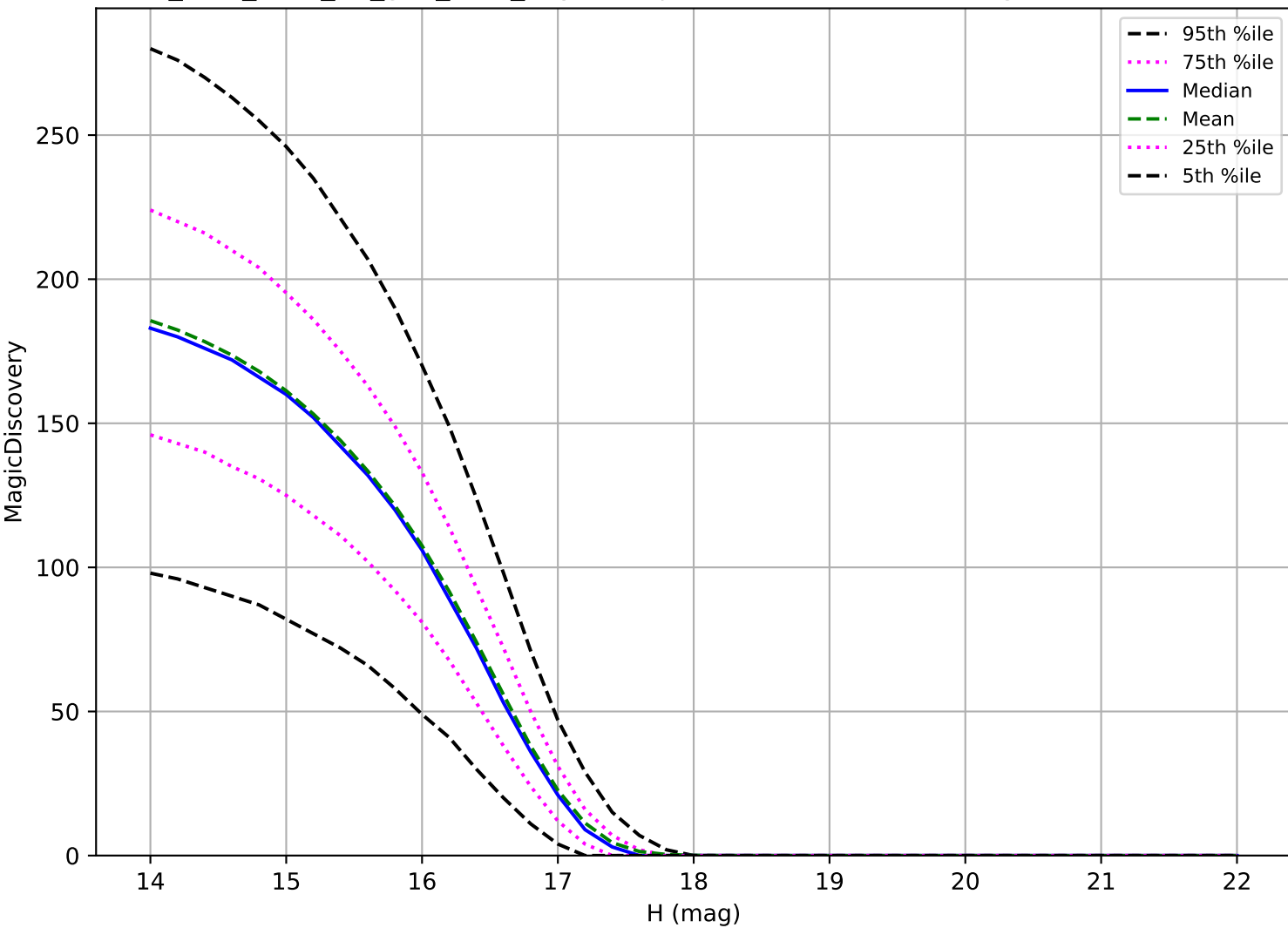
too_elab_r128_d2_griz_v3.4_10yrs: Trojan 6 detections in 60 nights detection loss
