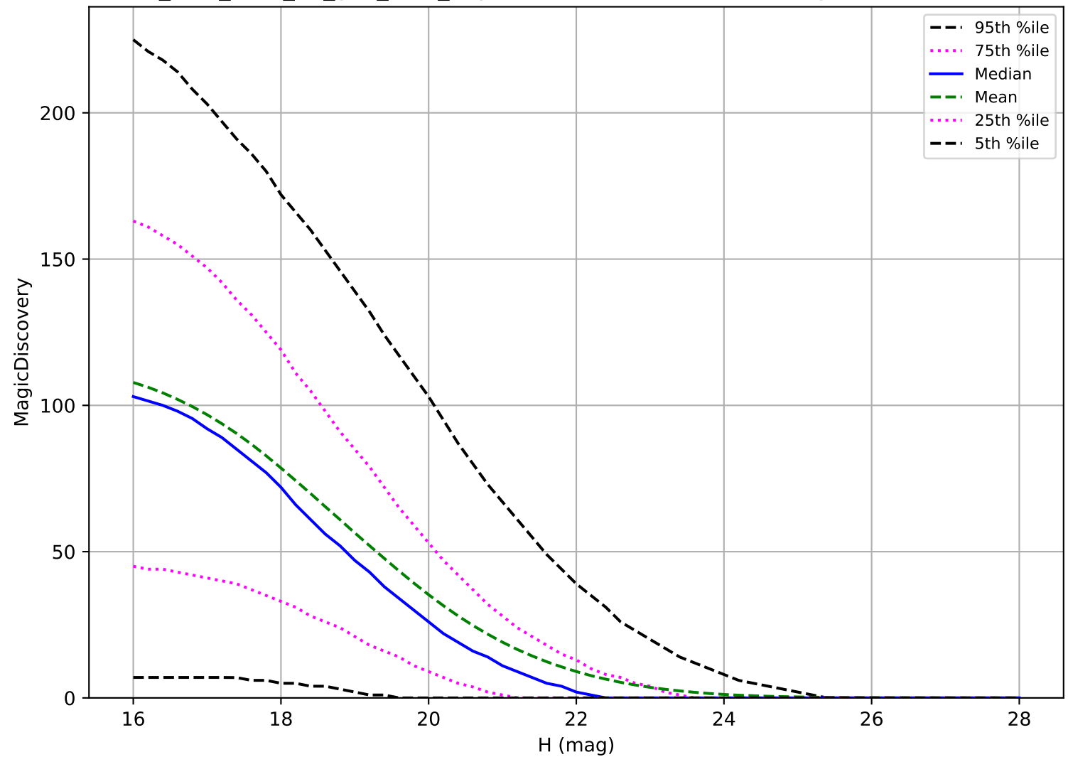
too_elab_r128_d2_griz_v3.4_10yrs: PHA 6 detections in 60 nights detection loss
