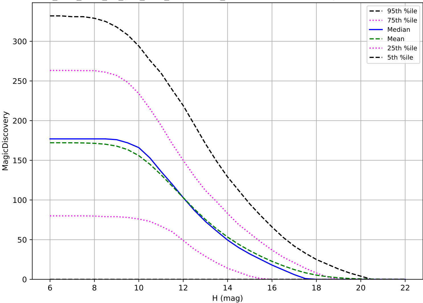
too_elab_r128_d2_griz_v3.4_10yrs: OCC_r5 6 detections in 60 nights detection loss
