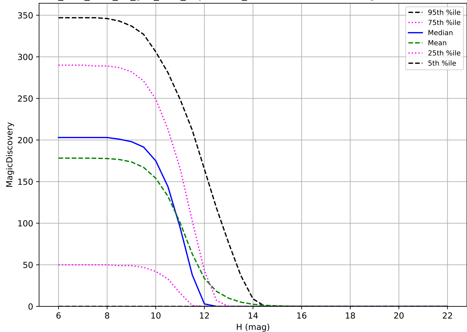
too_elab_r128_d2_griz_v3.4_10yrs: OCC_r20 6 detections in 60 nights detection loss
