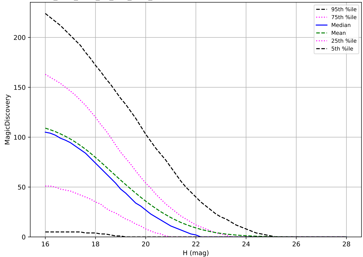
too_elab_r128_d2_griz_v3.4_10yrs: NEO 6 detections in 60 nights detection loss
