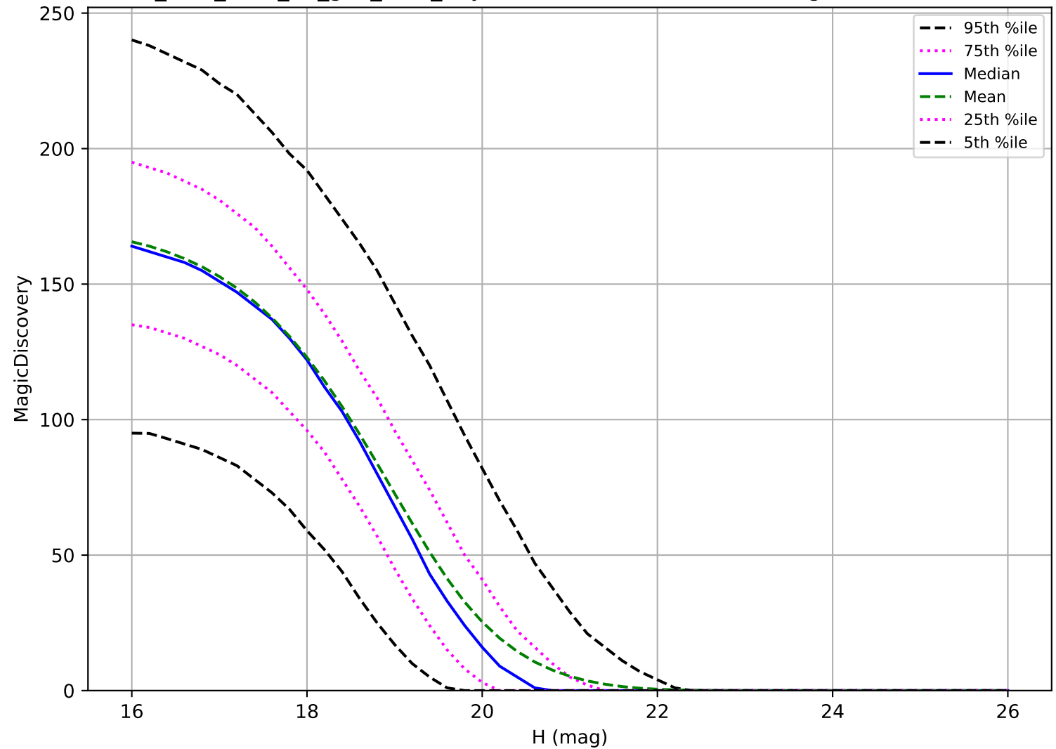
too_elab_r128_d2_griz_v3.4_10yrs: MBA 6 detections in 60 nights detection loss
