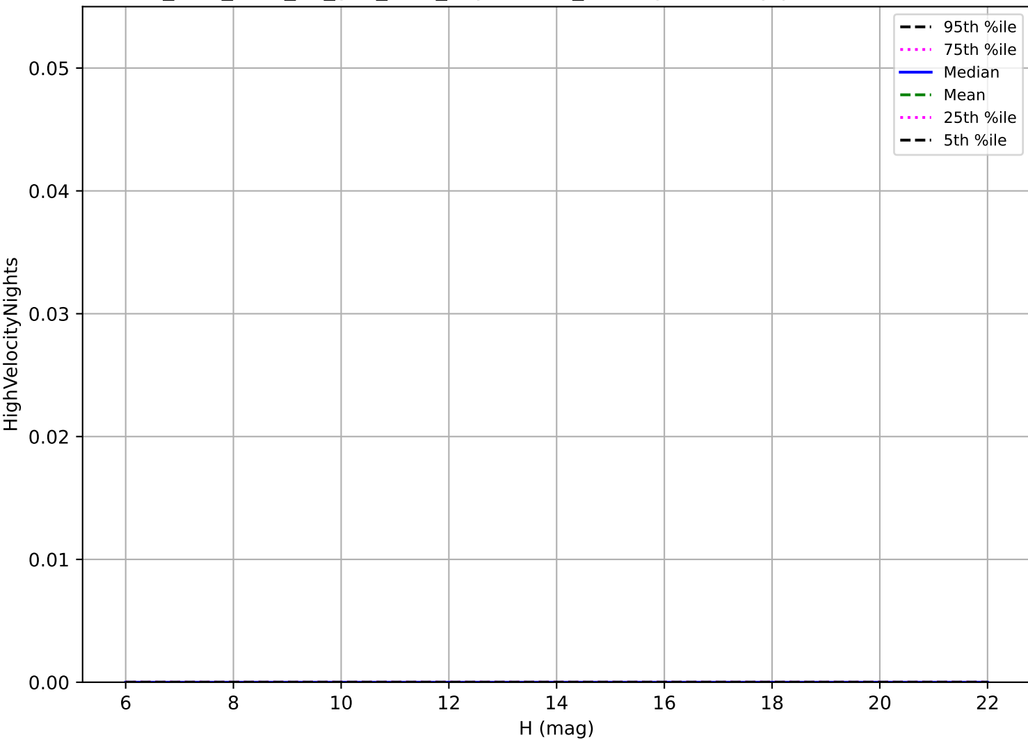
too_elab_r128_d2_griz_v3.4_10yrs: OCC_r20 High velocity pair detection loss
