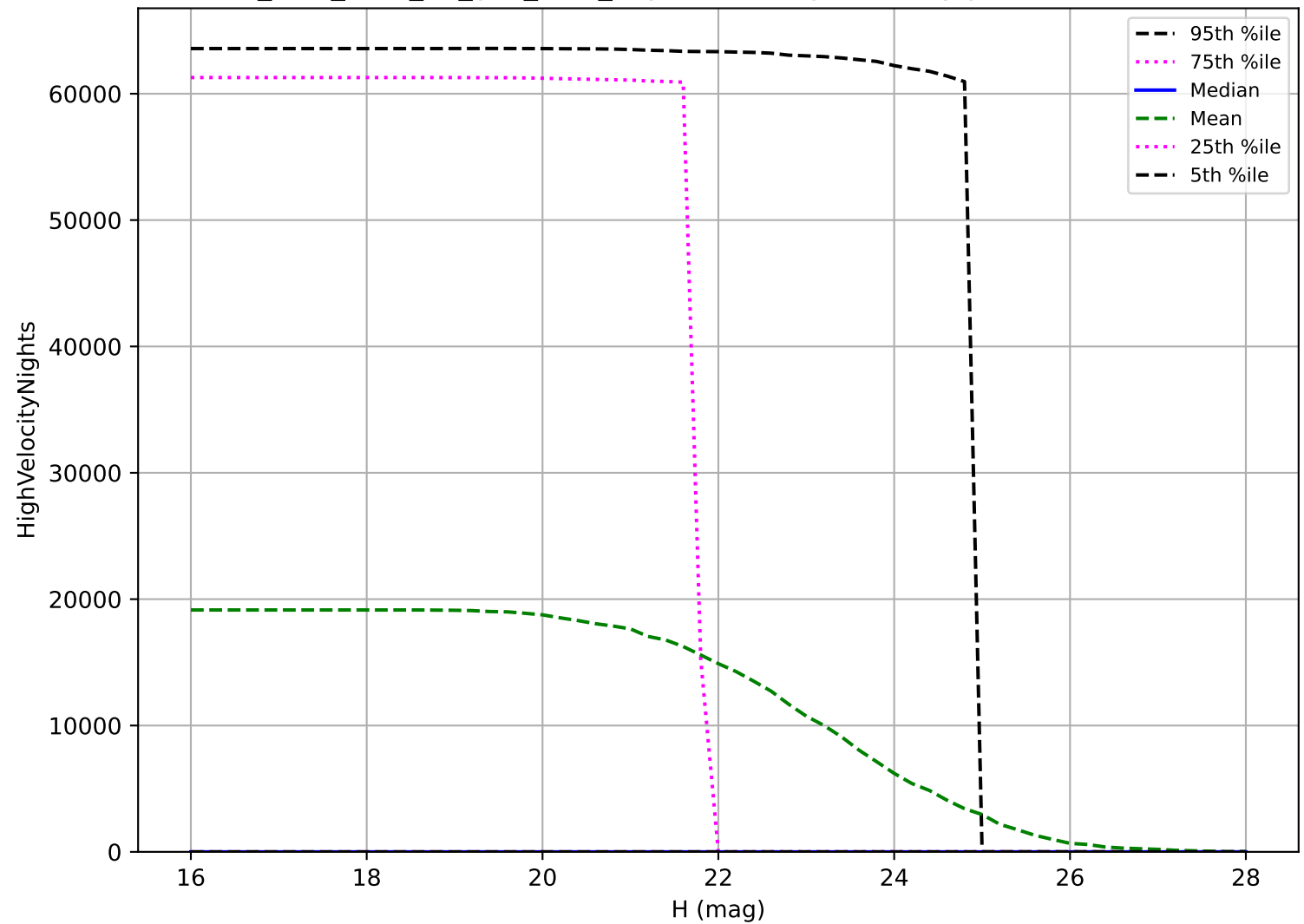
too_elab_r128_d2_griz_v3.4_10yrs: NEO High velocity pair detection loss
