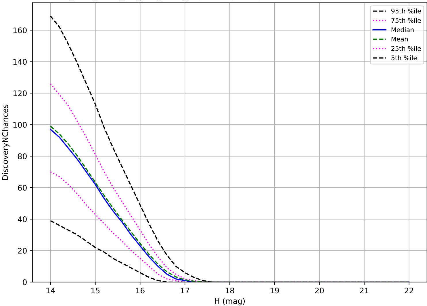
too_elab_r128_d2_griz_v3.4_10yrs: Trojan 3 pairs in 15 nights detection loss
