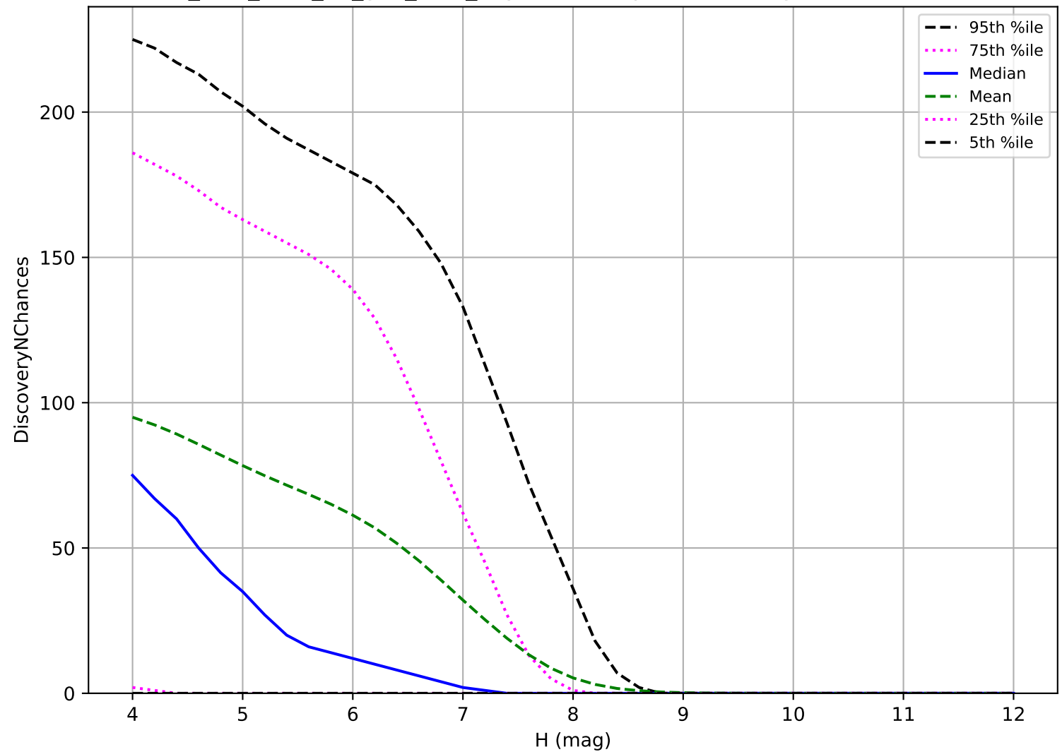
too_elab_r128_d2_griz_v3.4_10yrs: TNO 3 pairs in 15 nights detection loss
