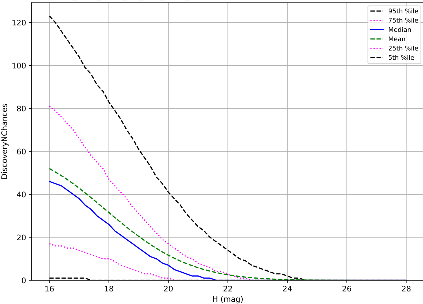
too_elab_r128_d2_griz_v3.4_10yrs: PHA 3 pairs in 15 nights detection loss
