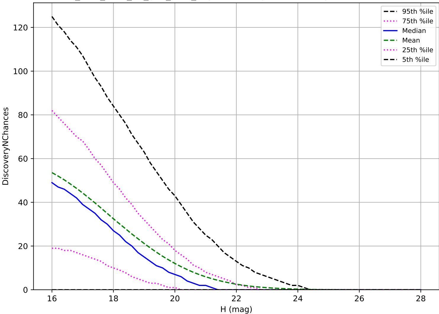
too_elab_r128_d2_griz_v3.4_10yrs: NEO 3 pairs in 15 nights detection loss
