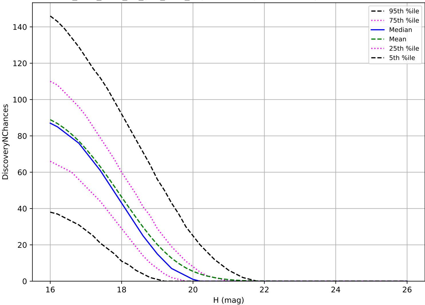
too_elab_r128_d2_griz_v3.4_10yrs: MBA 3 pairs in 15 nights detection loss
