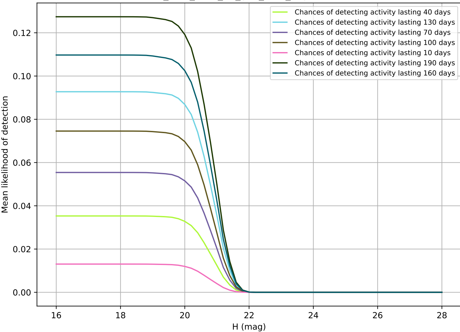
too_elab_r128_d2_griz_v3.4_10yrs Vatira
