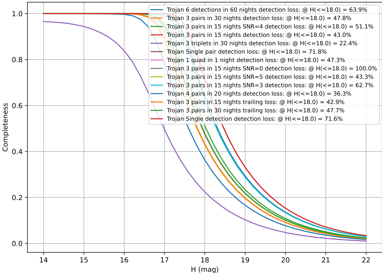
too_elab_r128_d2_griz_v3.4_10yrs: CumulativeCompleteness
