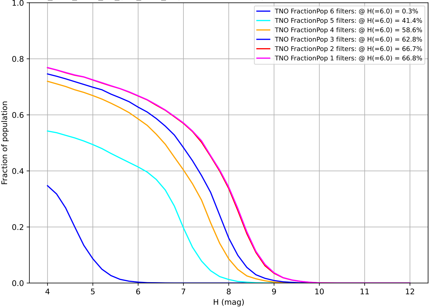
too_elab_r128_d2_griz_v3.4_10yrs: Fraction of population with colors in X filters TNO
