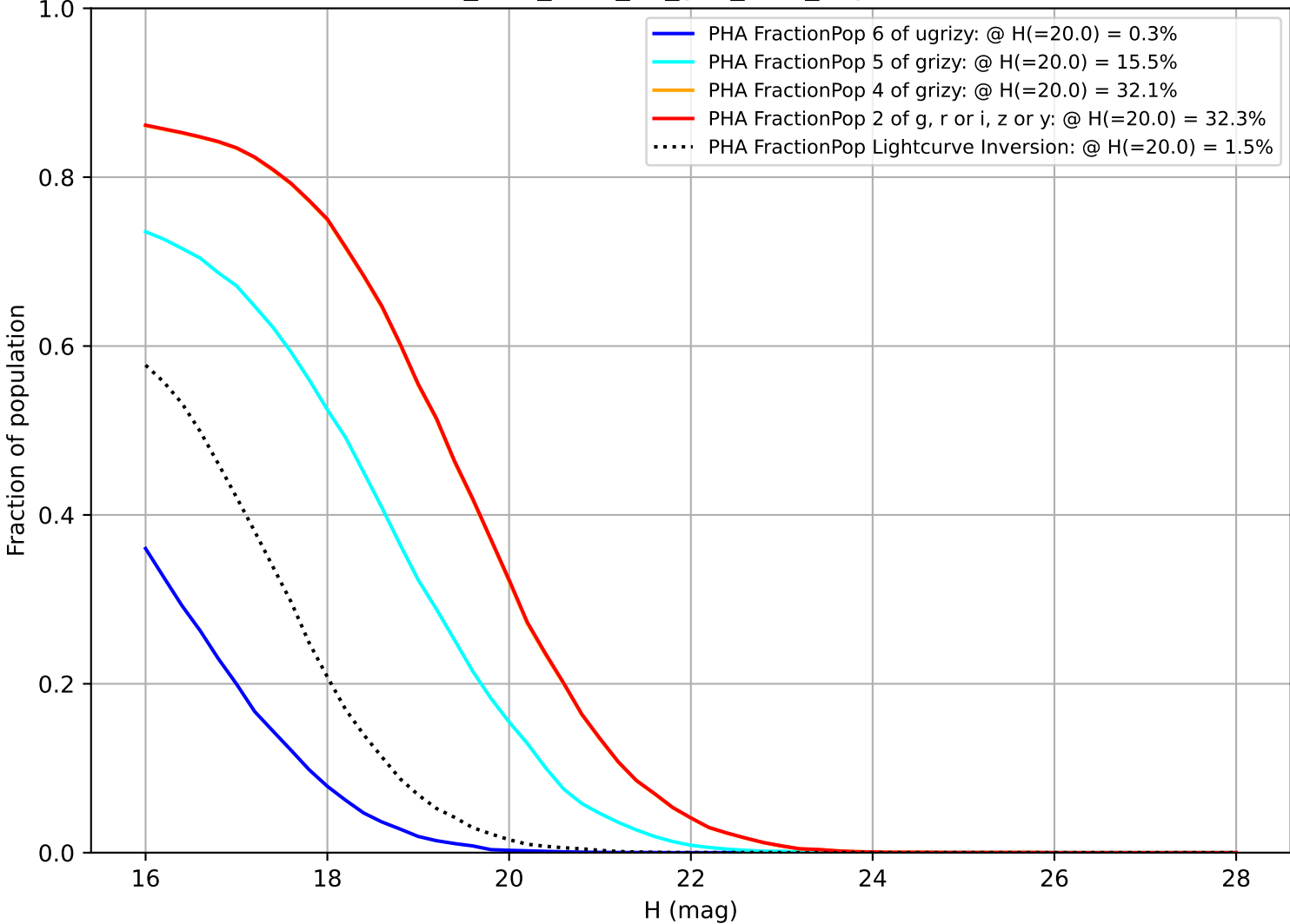
too_elab_r128_d2_griz_v3.4_10yrs PHA
