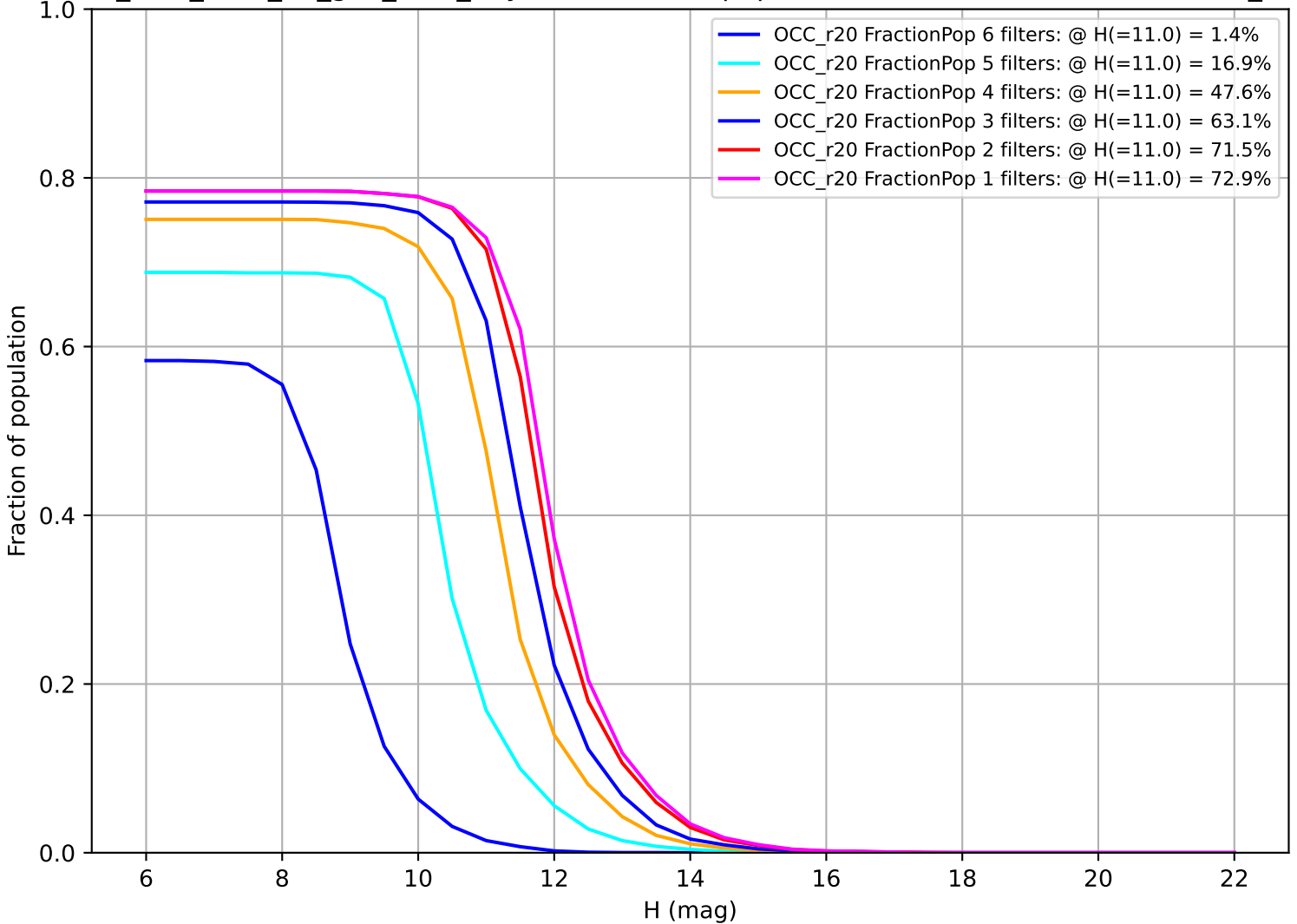
too_elab_r128_d2_griz_v3.4_10yrs: Fraction of population with colors in X filters OCC_r20
