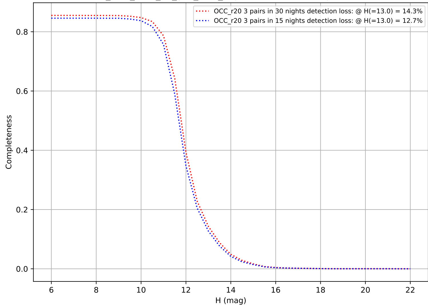
too_elab_r128_d2_griz_v3.4_10yrs: DifferentialCompleteness
