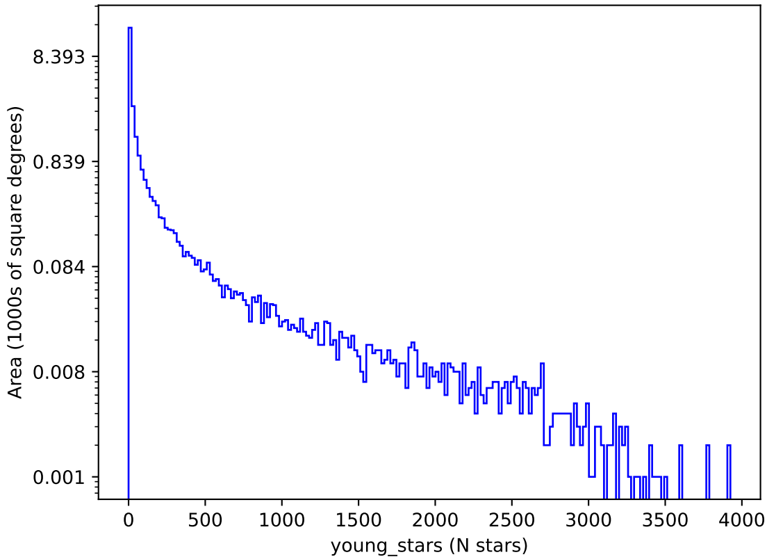
too_elab_r128_d2_griz_v3.4_10yrs : young_stars
