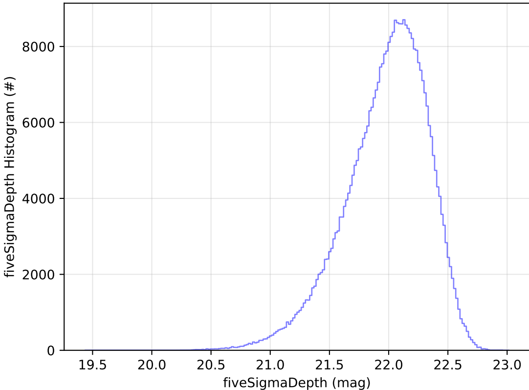
too_elab_r128_d2_griz_v3.4_10yrs y: fiveSigmaDepth Histogram
