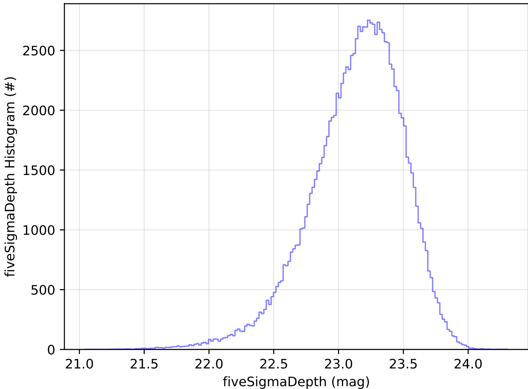
too_elab_r128_d2_griz_v3.4_10yrs u: fiveSigmaDepth Histogram
