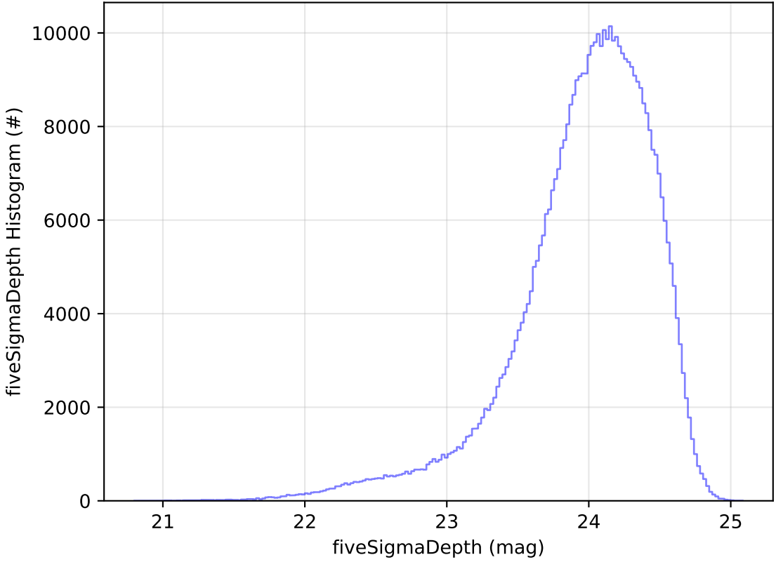
too_elab_r128_d2_griz_v3.4_10yrs r: fiveSigmaDepth Histogram
