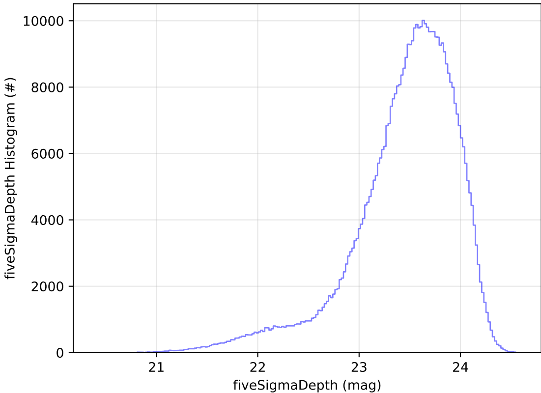
too_elab_r128_d2_griz_v3.4_10yrs i: fiveSigmaDepth Histogram
