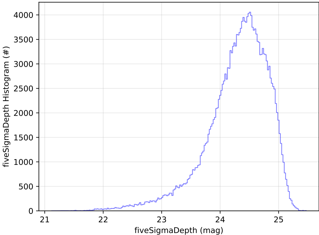
too_elab_r128_d2_griz_v3.4_10yrs g: fiveSigmaDepth Histogram
