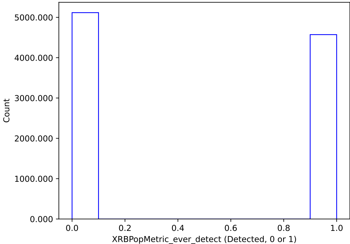
too_elab_r128_d2_griz_v3.4_10yrs : XRBPoMetric_ever_detect
