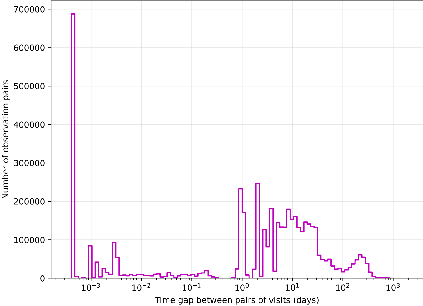
too_elab_r128_d2_griz_v3.4_10yrs z band: Tgaps observationStartMJD
