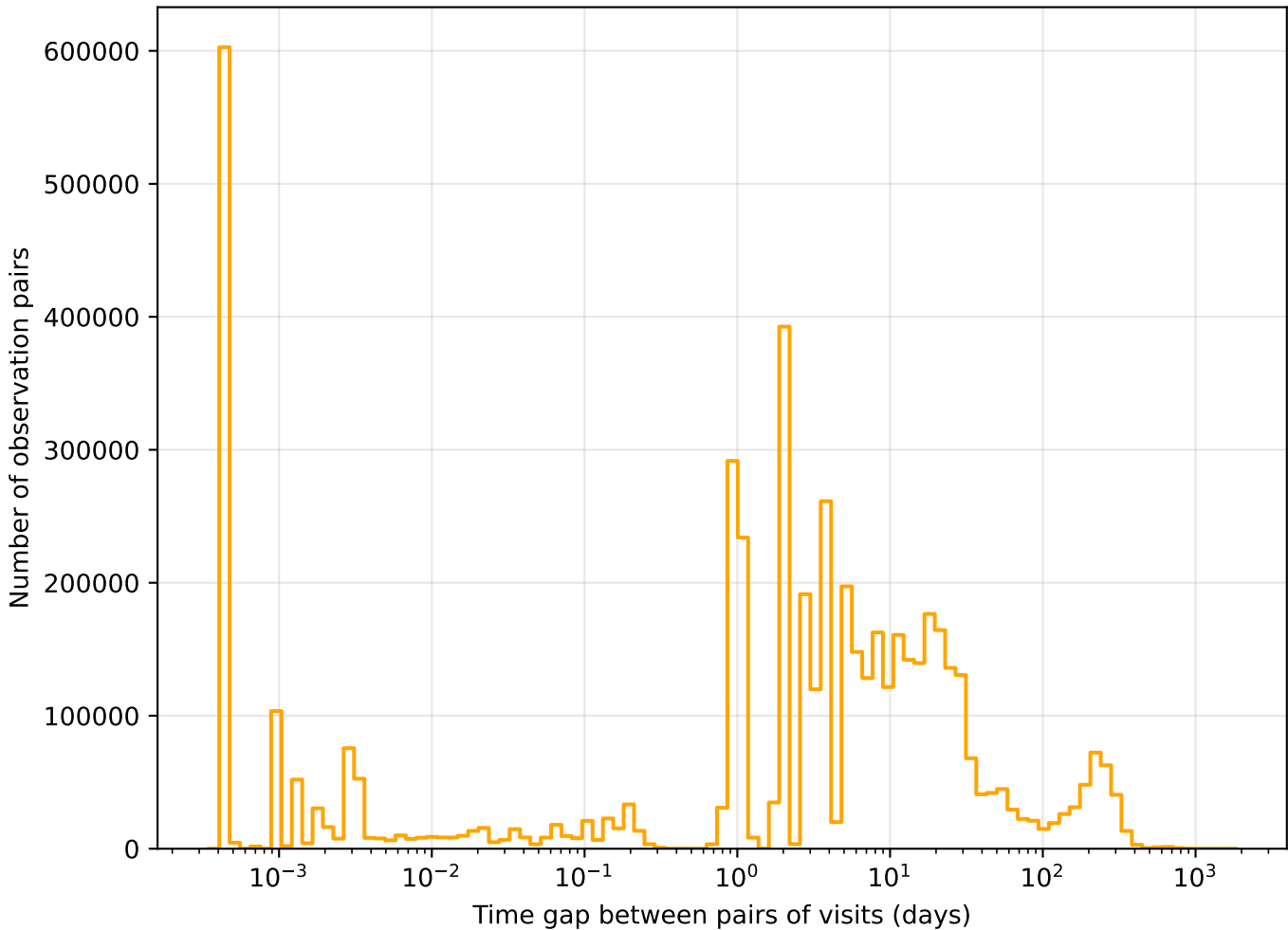
too_elab_r128_d2_griz_v3.4_10yrs r band: Tgaps observationStartMJD
