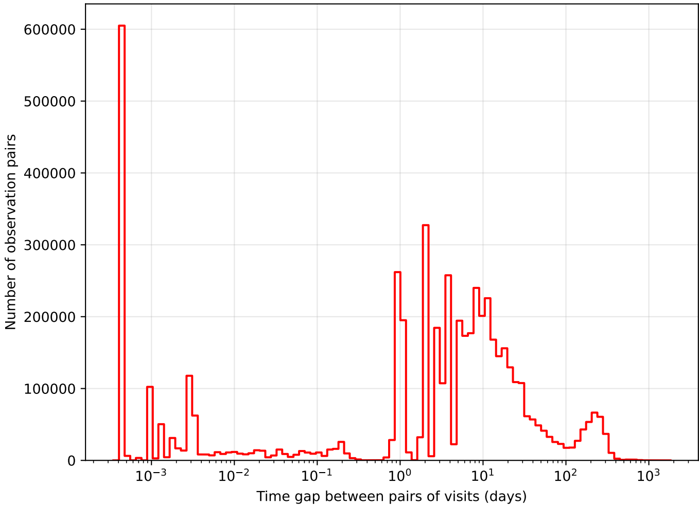
too_elab_r128_d2_griz_v3.4_10yrs i band: Tgaps observationStartMJD
