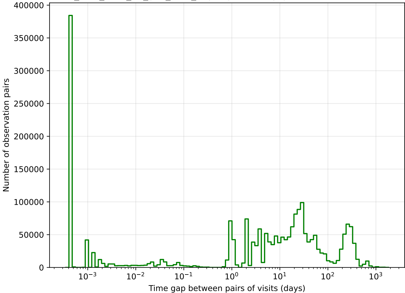
too_elab_r128_d2_griz_v3.4_10yrs g band: Tgaps observationStartMJD
