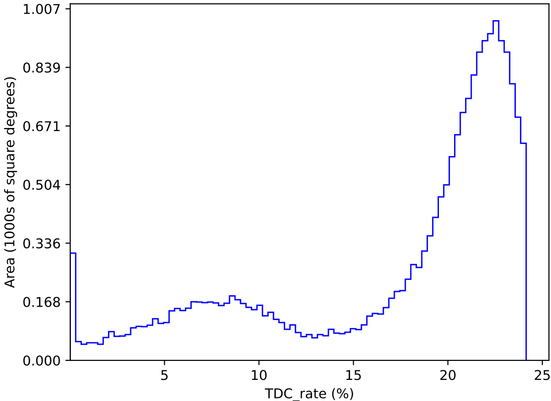
too_elab_r128_d2_griz_v3.4_10yrs : TDC_rate
